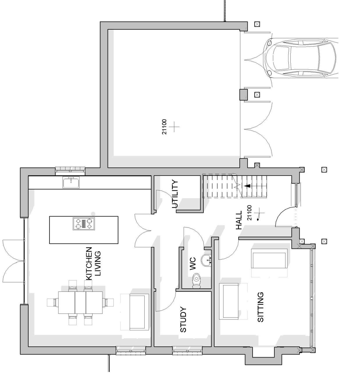
Plot 3 - Ground Floor Plan as Proposed
